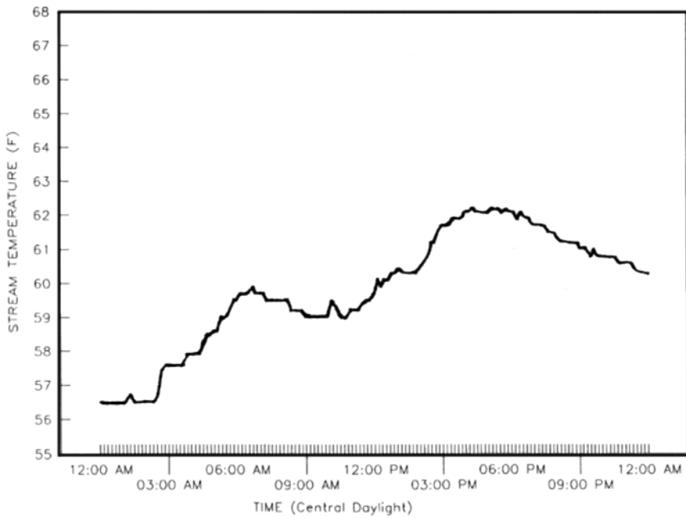
Figure 6 Quarry Road Thermograph Kinnickinnic River at Quarry Road July 25, 1993
